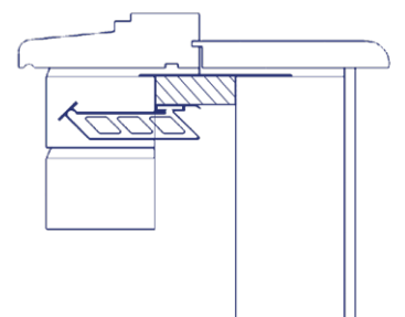
Sill detail
