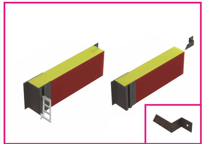
FR60+ Profile | 150mm - 300mm cavities
