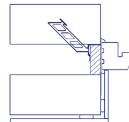
Fig.1 Flush jamb
