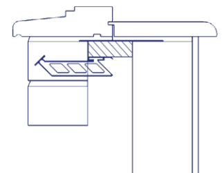
Sill detail
