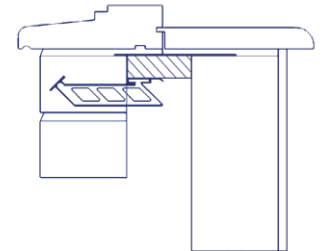
Sill detail
