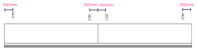
FR60+ fixing flanges installation
