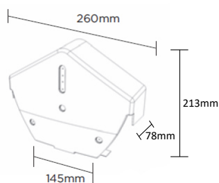
Universal dry fix angled ridge end cap
